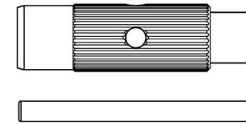
5.5 & 7.0 Alum. wrench 鋁合金套筒工具 (700003)
