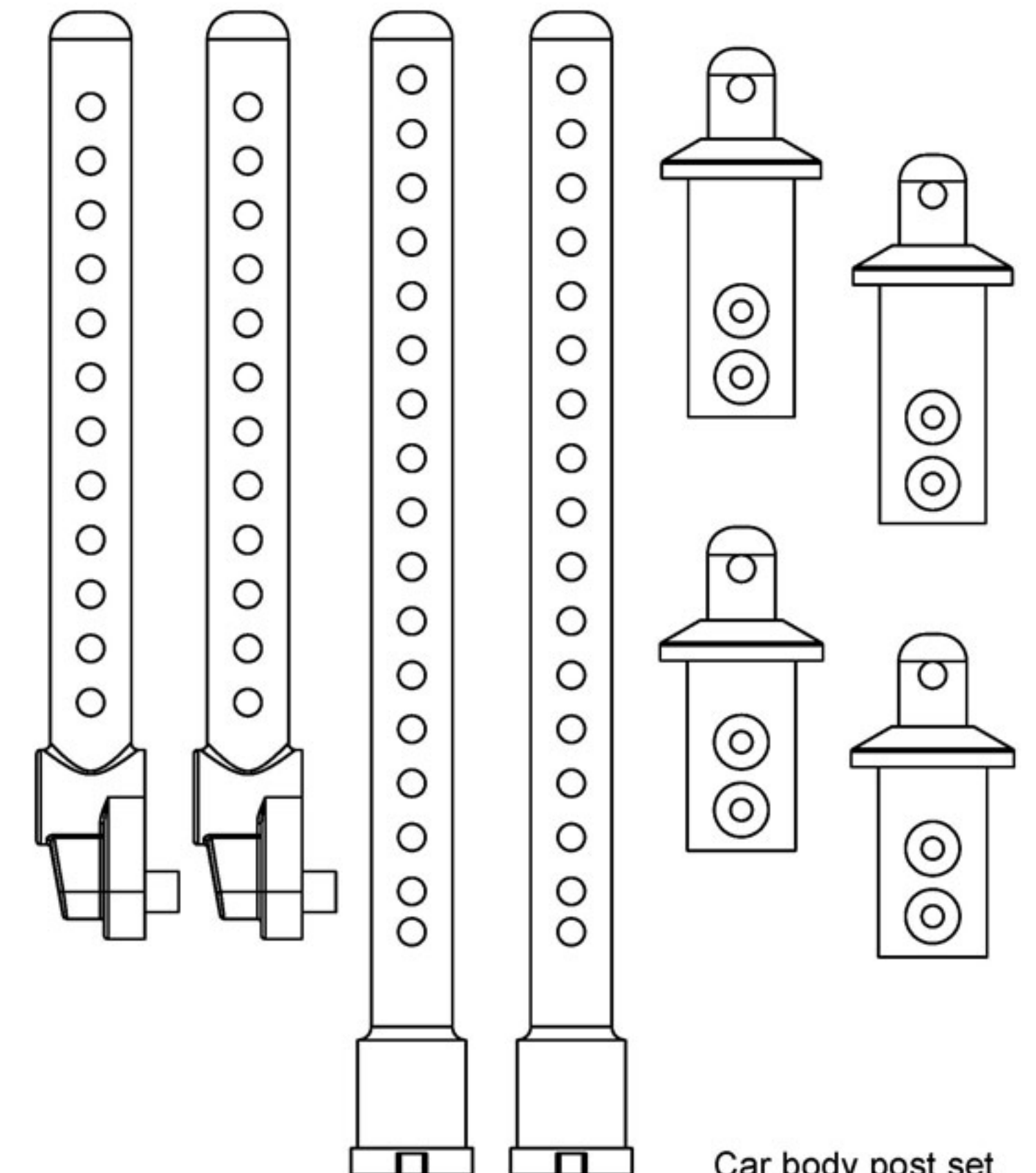
Car body post set 車殼支柱組 210381
