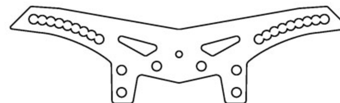
XXX Carbon wide front damper stay 碳纖維寬形前避震架 210380
