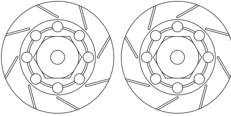
Wheel huds w/disc shape 碟型六角輪座組 210043
