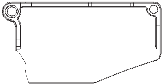
Wheel huds w/disc shape 碟型六角輪座組 210043
