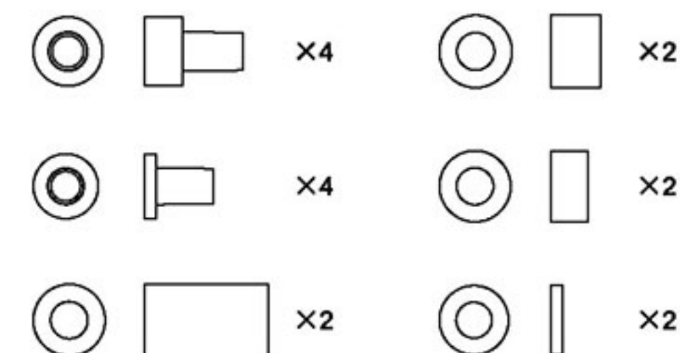
Shaft bush & spacer set (white) 襯套墊片組 (白) 210063W
