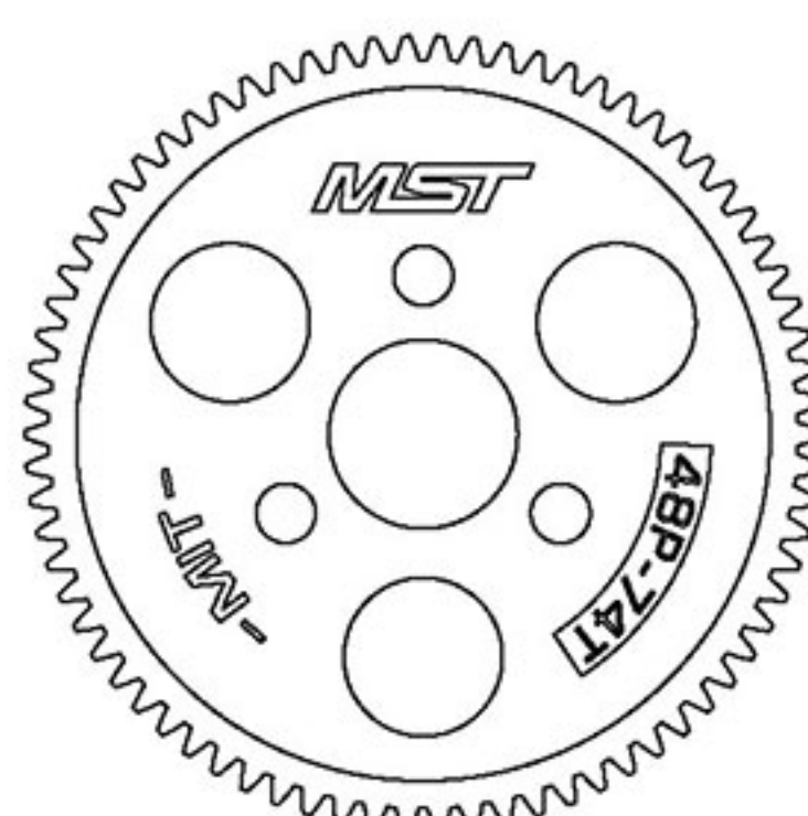
Spur gear 48P-74T 大直齒 48P-74T 210096
